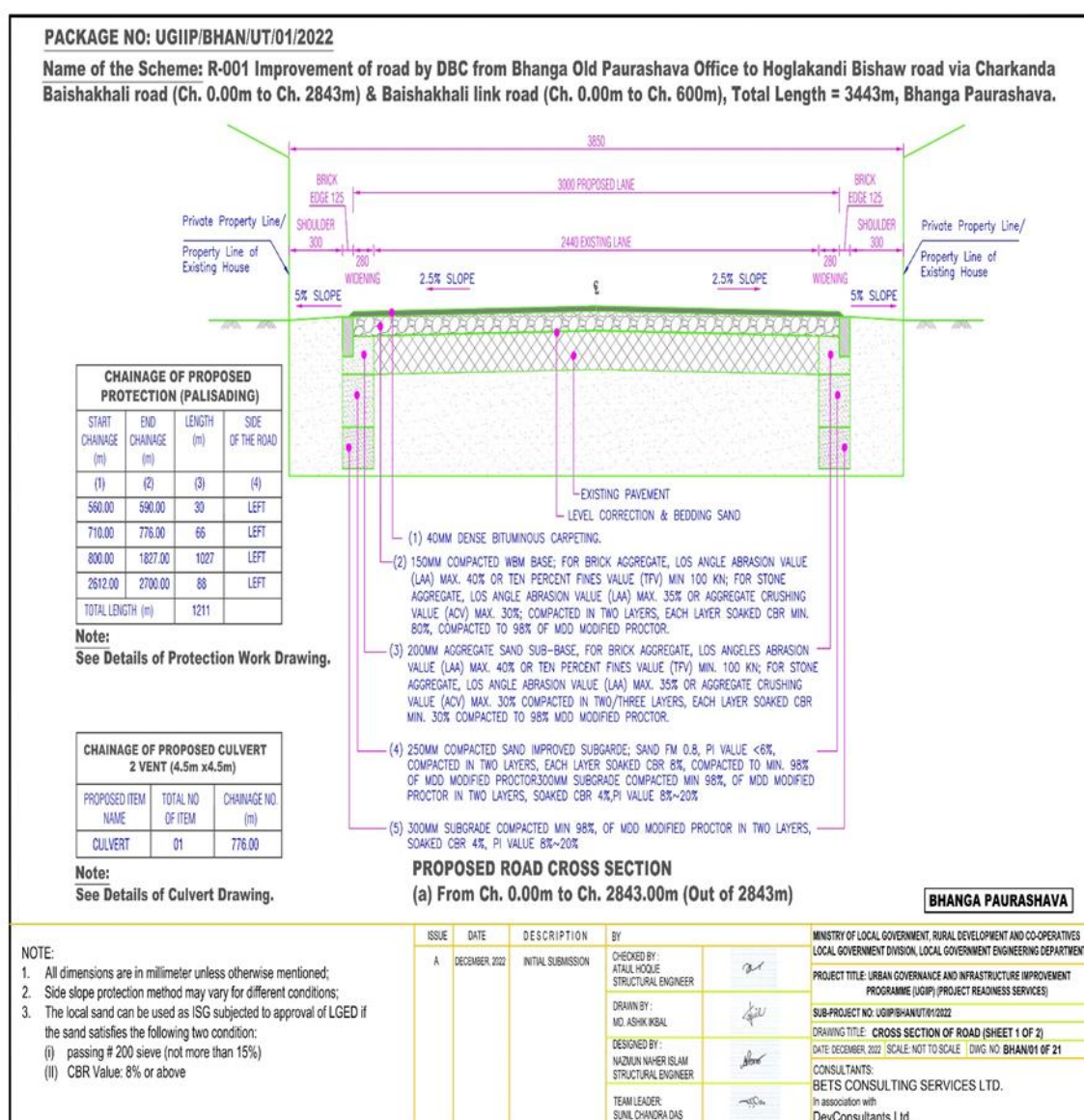
Figure 5: Cross-Section of Road in Bhanga Pourashava
