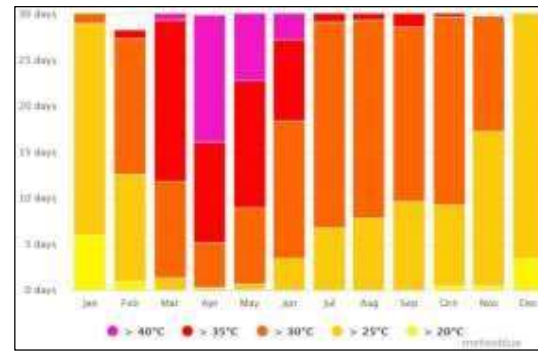
Maximum Temperatures
