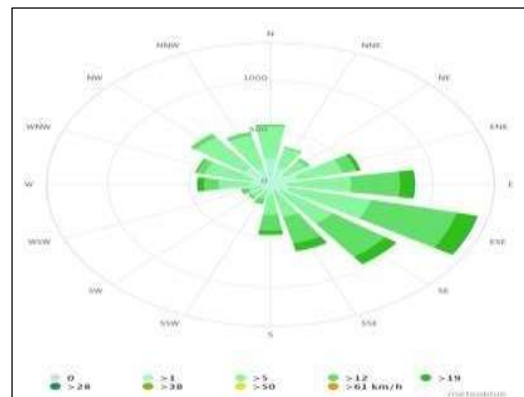
Wind rose
