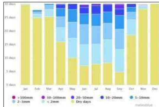
Precipitation Amounts
