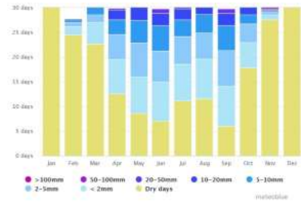
Precipitation Amounts
