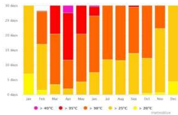
Maximum Temperatures
