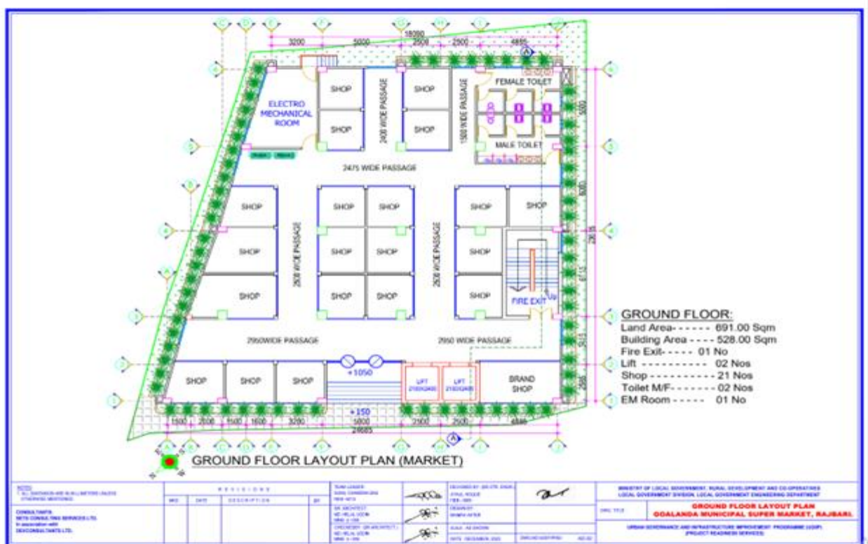
Figure 7: Ground Floor of proposed marker in goalanda pauroshava
