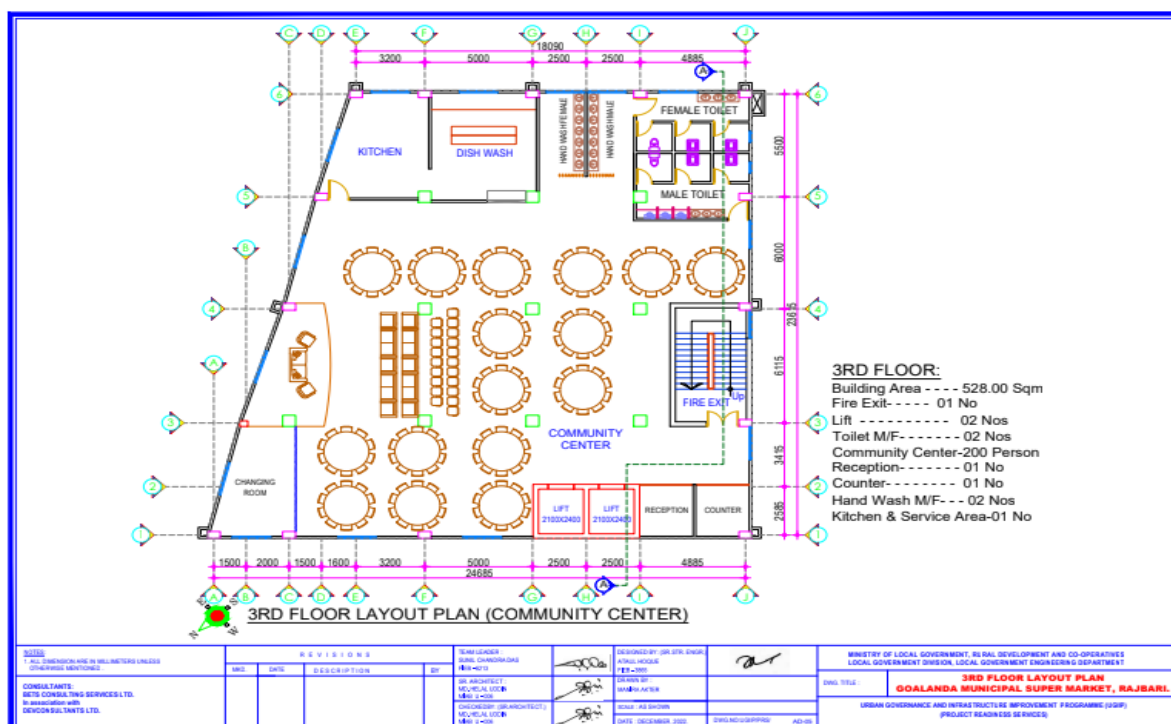
Figure 10: 3rd floor of proposed marker in goalanda pauroshava
