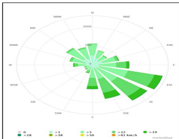
Wind Speed
