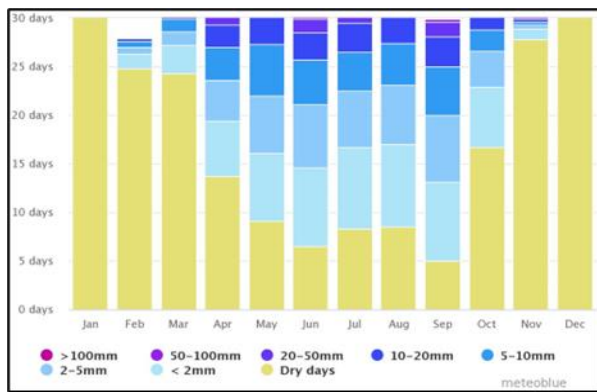
Precipitation Amounts
