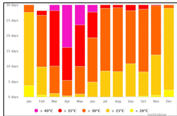
Maximum Temperature
