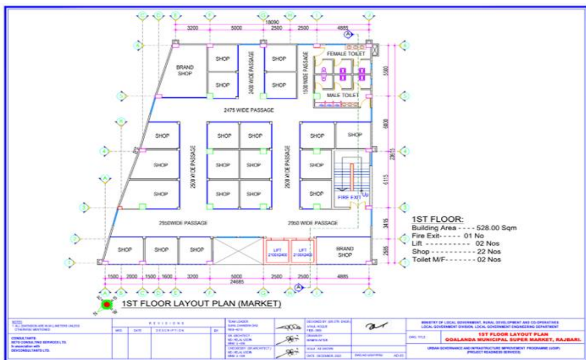
Figure 8: 1st floor of proposed marker in goalanda pauroshava
