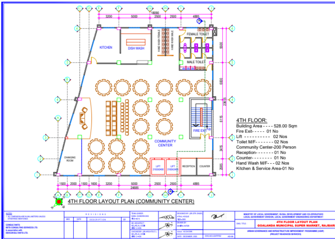
Figure 11: 4th floor of proposed marker in goalanda pauroshava
