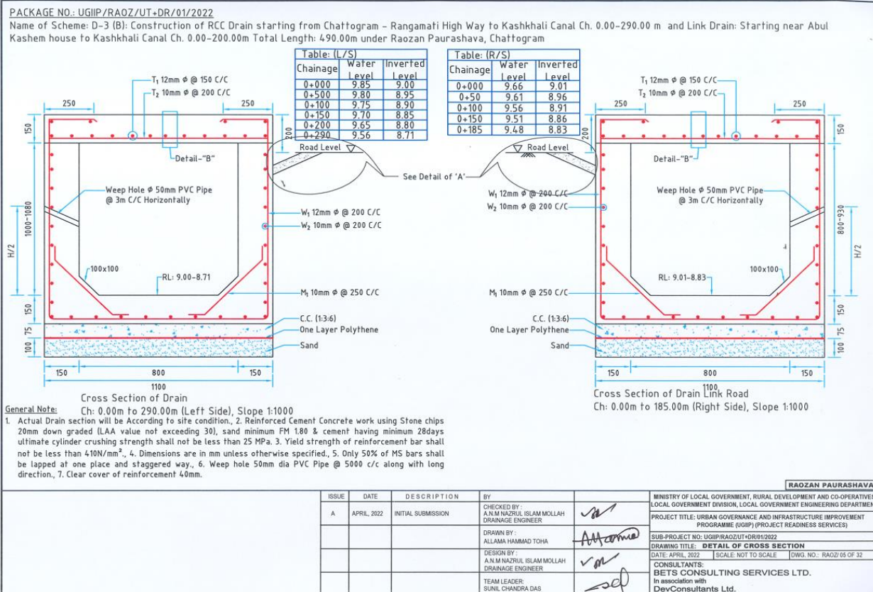
Figure III-IV: Cross-Section of Drain
