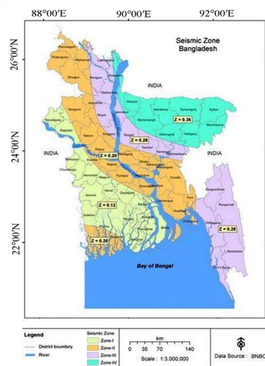
Figure IV-5: Seismic Zones of Bangladesh (4 Zones)
